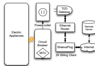
Figure 1. Our architecture using TED monitors/gateways and SheevaPlug computers.
