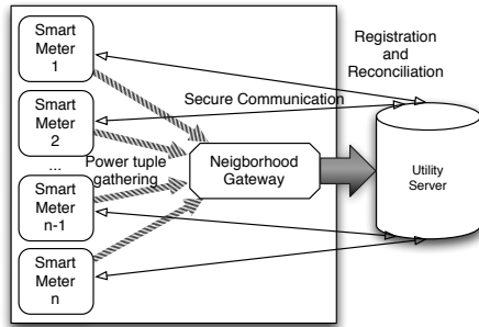
Figure 8. Privacy-enhanced smart metering using neighborhood gateways.
